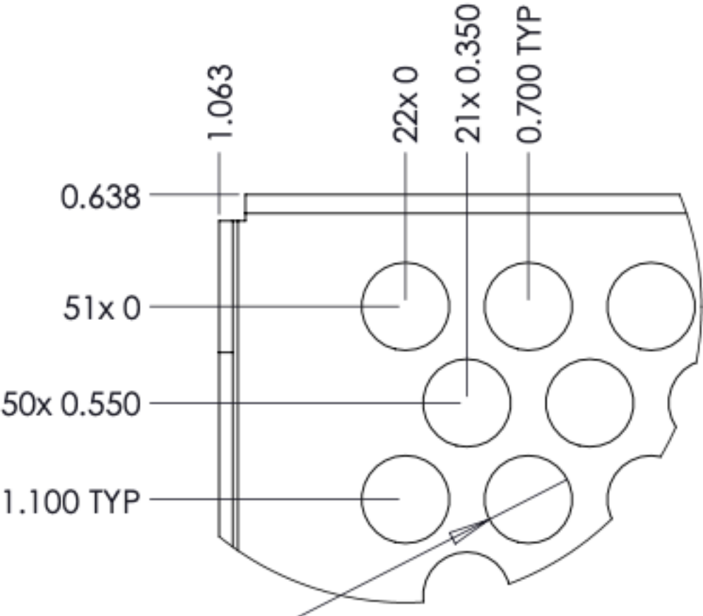
DETAIL L SCALE 1 : 1
